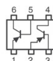
XP0643500L Panasonic Electronic Components TRANS 2PNP 20V 0.03A SMINI6
