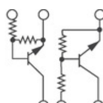
XP0621300L Panasonic Electronic Components TRANS PREBIAS DUAL NPN SMINI6
