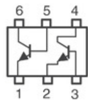
XP0650100L Panasonic Electronic Components TRANS 2NPN 50V 0.1A SMINI6
