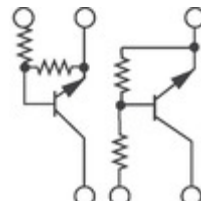
XP0621000L Panasonic Electronic Components TRANS PREBIAS DUAL NPN SMINI6
