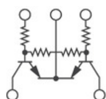
XP0121100L Panasonic Electronic Components TRANS 2NPN PREBIAS 0.15W SMINI5
