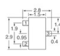
DRA2114E0L Panasonic Electronic Components TRANS PREBIAS PNP 200MW MINI3
