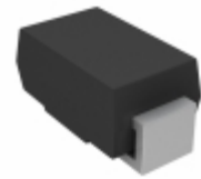
SMAJ6.5A-M3/5A Vishay Semiconductor Diodes Division TVS DIODE 6.5VWM 11.2VC DO-214AC
