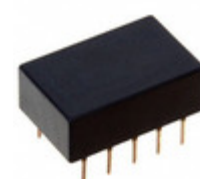
TQ2-L2-12V-3 Panasonic Electric Works RELAY TELECOM DPDT 1A 12V
