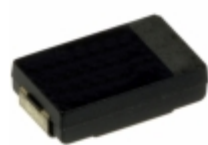
EEF-CX0G221XR Panasonic Electronic Components CAP ALUM POLY 220UF 20% 4V SMD
