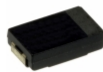
EEF-CX0G331R Panasonic Electronic Components CAP ALUM POLY 330UF 20% 4V SMD
