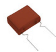
ECW-F2125HAQ Panasonic Electronic Components CAP FILM 1.2UF 3% 250VDC RADIAL
