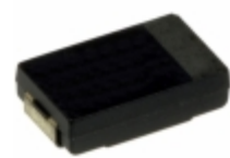
EEF-CX0G181XR Panasonic Electronic Components CAP ALUM POLY 180UF 20% 4V SMD
