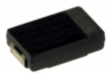
EEF-CX0E471R Panasonic Electronic Components CAP ALUM POLY 470UF 20% 2.5V SMD
