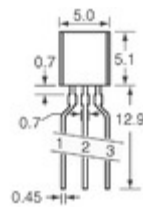
2SA07200RA Panasonic Electronic Components TRANS PNP 70V 0.5A TO-92
