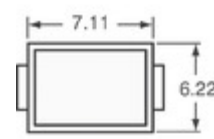
SMCJ85CA-TP Micro Commercial Co TVS DIODE 85VWM 137VC SMC
