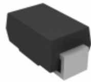
SMAJ100A-M3/61 Vishay Semiconductor Diodes Division TVS DIODE 100VWM 162VC DO-214AC
