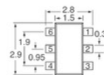
MA6X12500L Panasonic Electronic Components DIODE ARRAY GP 40V 100MA MINI6
