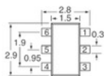
MA6X12900L Panasonic Electronic Components DIODE ARRAY GP 200V 200MA MINI6
