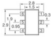
MA6X12800L Panasonic Electronic Components DIODE ARRAY GP 80V 100MA MINI6
