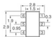
MA6X12600L Panasonic Electronic Components DIODE ARRAY GP 80V 100MA MINI6
