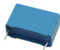
B32523Q3684K EPCOS (TDK) CAP FILM 0.68UF 10% 250VDC RAD
