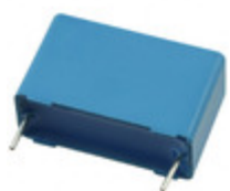
B32523Q3474K189 EPCOS (TDK) CAP FILM 0.47UF 10% 250VDC RAD
