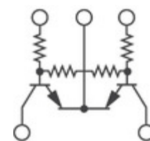
XP0121500L Panasonic Electronic Components TRANS 2NPN PREBIAS 0.15W SMINI5
