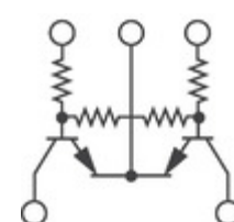
XP0121600L Panasonic Electronic Components TRANS 2NPN PREBIAS 0.15W SMINI5
