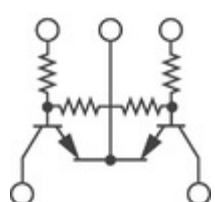
XP0121200L Panasonic Electronic Components TRANS 2NPN PREBIAS 0.15W SMINI5
