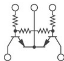
XP0121400L Panasonic Electronic Components TRANS 2NPN PREBIAS 0.15W SMINI5
