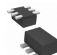
DMG964030R Panasonic Electronic Components TRANS PREBIAS NPN/PNP SSMINI6
