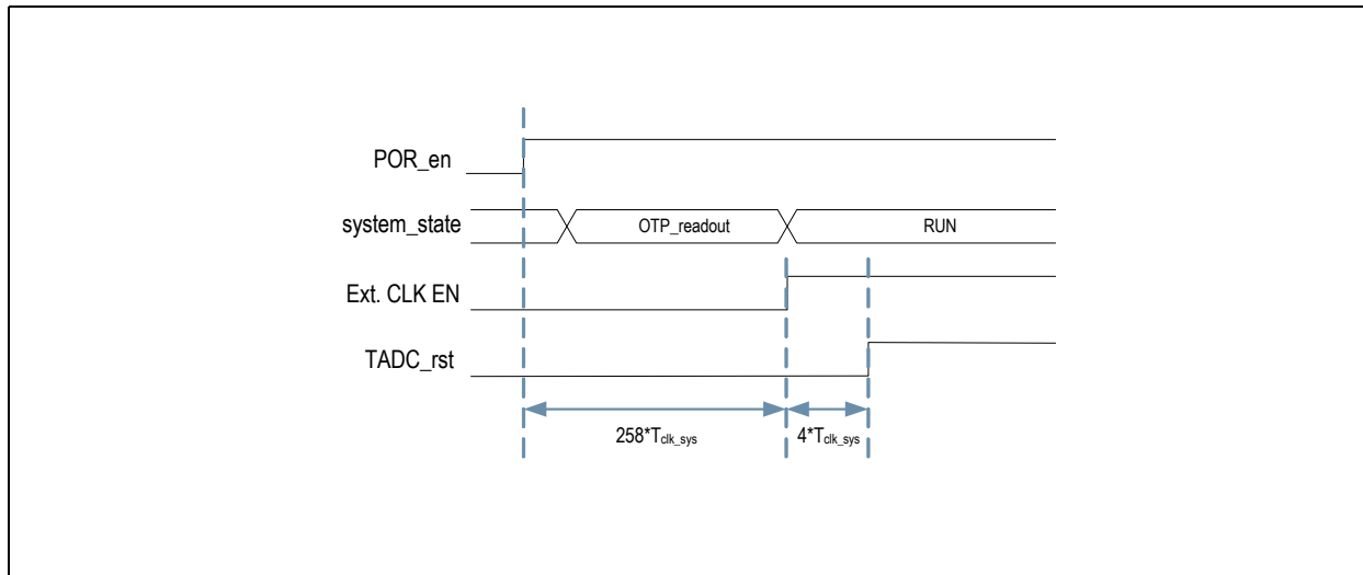
Figure 14. Start-up Procedure
