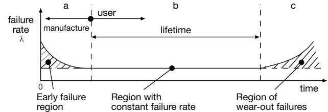
Fig. 11 - Failure rate ( \lambda ) as a function of time ("bath-tub life curve")
