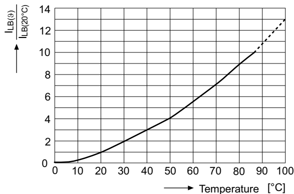
Fig. 9 - Typical variation of leakage current with temperature
