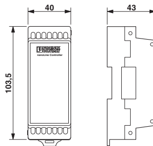
Dimensioned drawing
