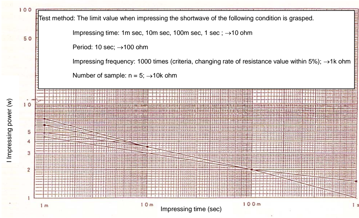
Fig.19. Pulse limited data of ERJ3G (1608)-type
